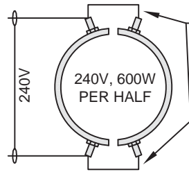
WIRED IN PARALLEL
