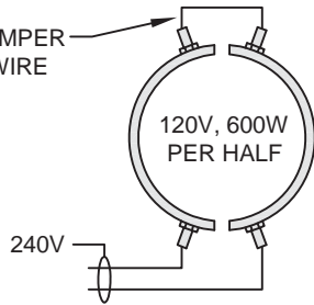
WIRED IN SERIES
