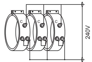
240V / 480V - Terminal Connection
