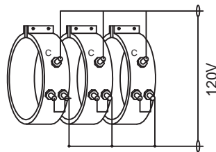
120V / 240V - Terminal Connection
