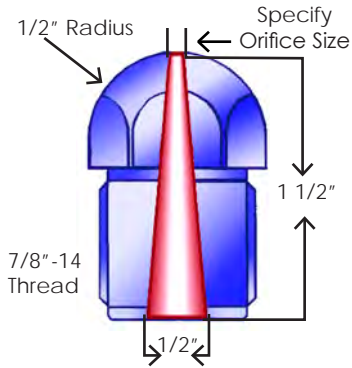
1/2" Radius
