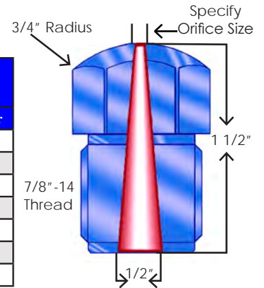
3/4" Radius
